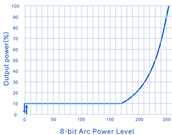
Logarithmic Dimming Curve:(DALI-2 Model
