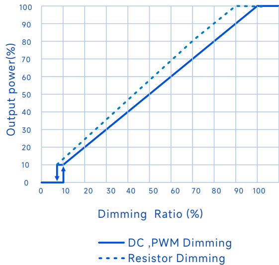
O/P Power Vs. Dimming
