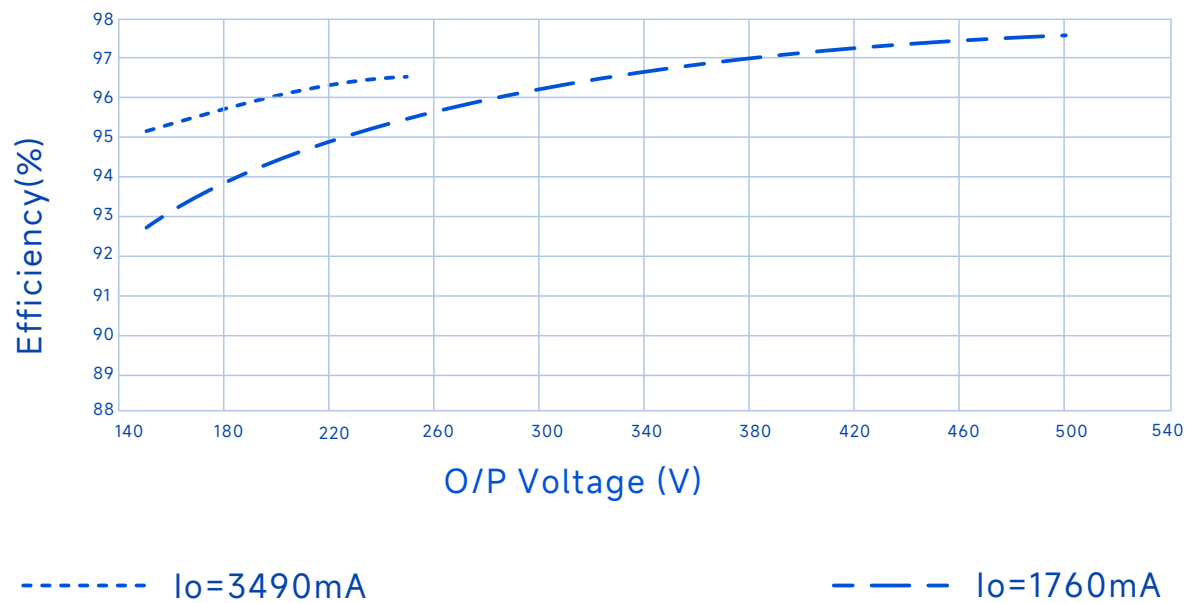
Efficiency Vs. O/P Voltage (Vin=480Vac)
