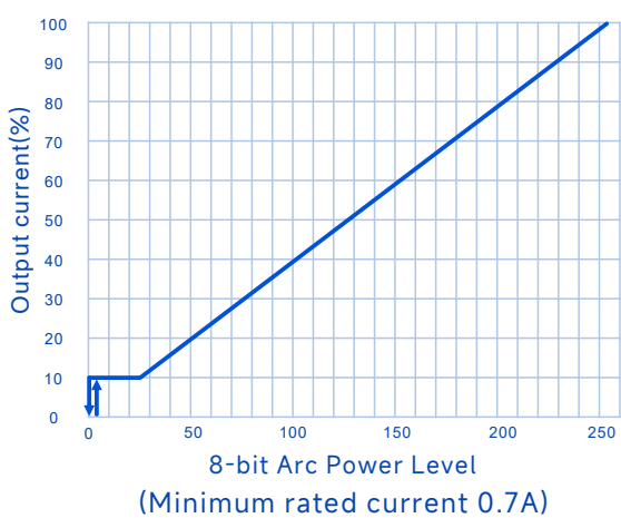
Linear Dimming Curve:(DMX Model)
